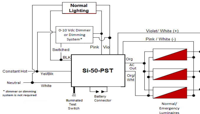
Typical Wiring Diagram
